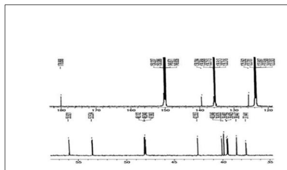
Fig. 2. 13 C-NMR spectrum of compound 3
