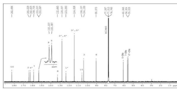
Fig. 4. 13 C-NMR spectrum of compound 7
