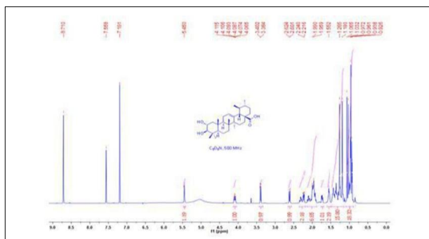
Fig. 1. 1 H-NMR spectrum of compound 3
