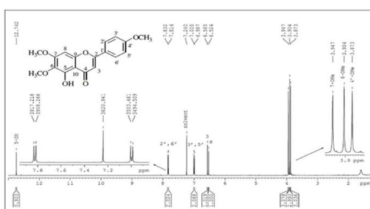
Fig. 3. 1 H-NMR spectrum of compound 7
